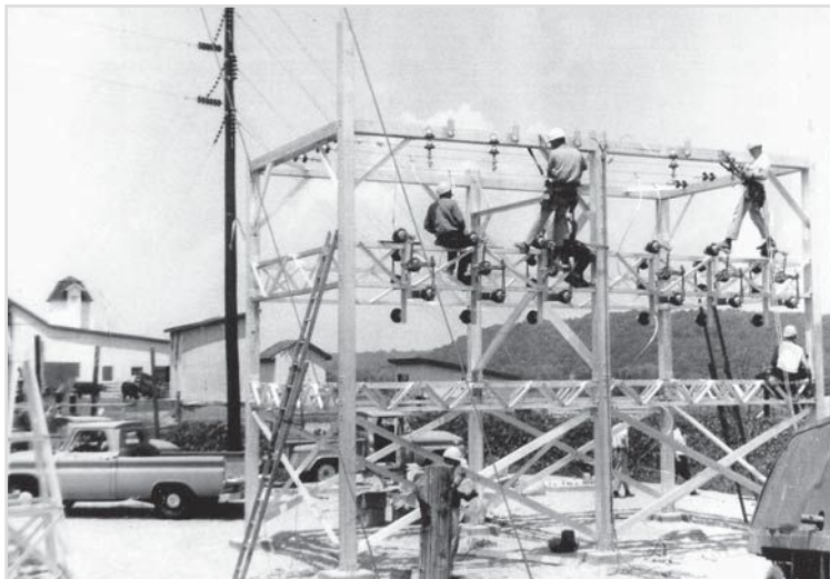
Hoosier Energy crews built and converted hundreds of substations in the 1970s.
