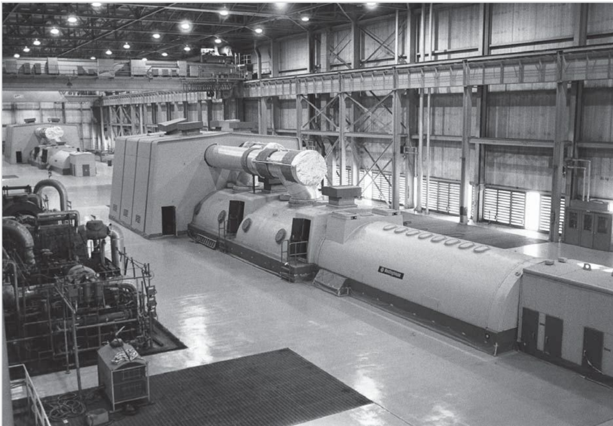
Merom Station's turbine-generators have performed yeoman-like service for Hoosier Energy since 1983 when the plant began operating.
