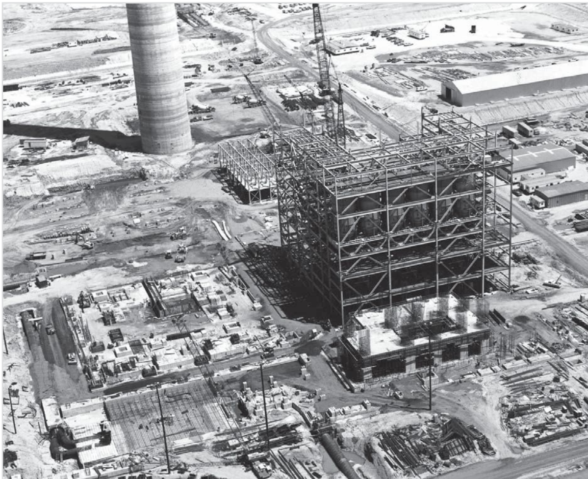
By 1982, structural steel was well on its way to topping out at the Merom Station's first unit. But demand for power had already begun to slip in Indiana and the U.S., and Hoosier Energy would be faced with the challenge of marketing surplus power from the plant.
